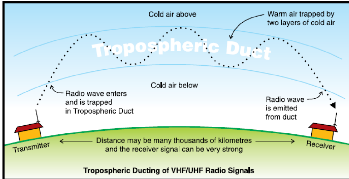
VHF and UHF radio waves can be caught in a tropospheric duct caused by a heat inversion layer in the lower atmosphere, (the troposphere).
